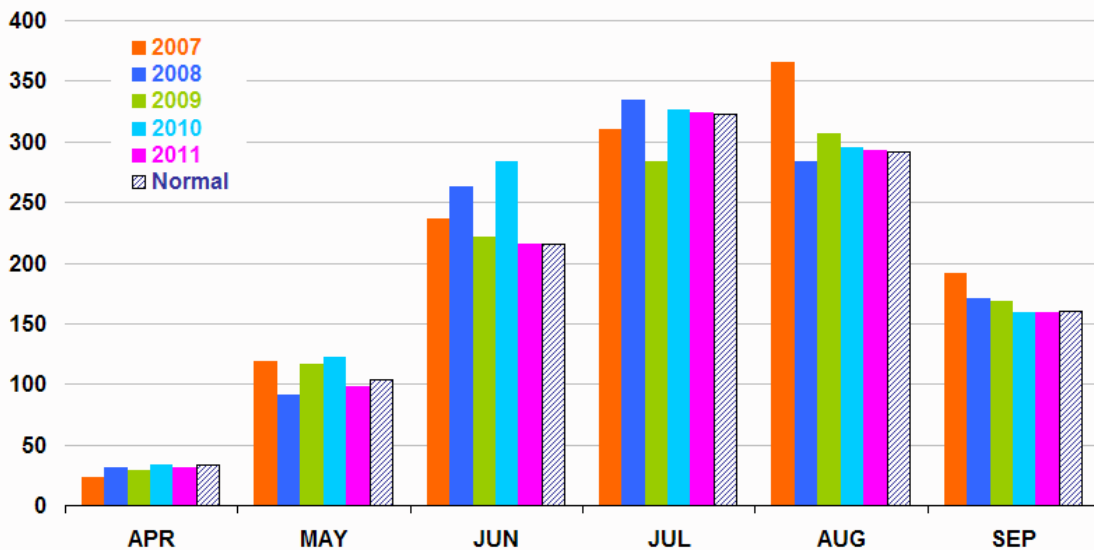
U.S. Summer Cooling Degree-Days (population-weighted)
