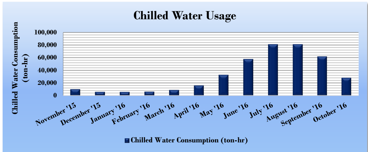
Figure 18 – Chilled Water Usage
