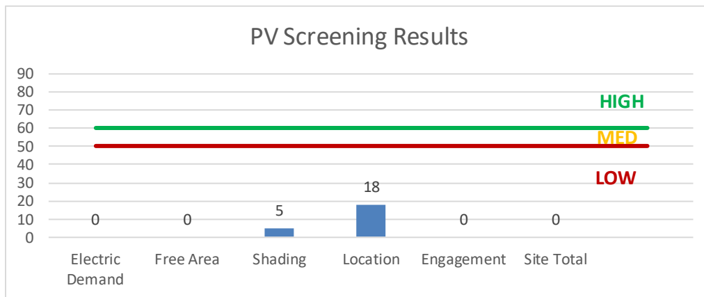
Figure 18 - Photovoltaic Screening
