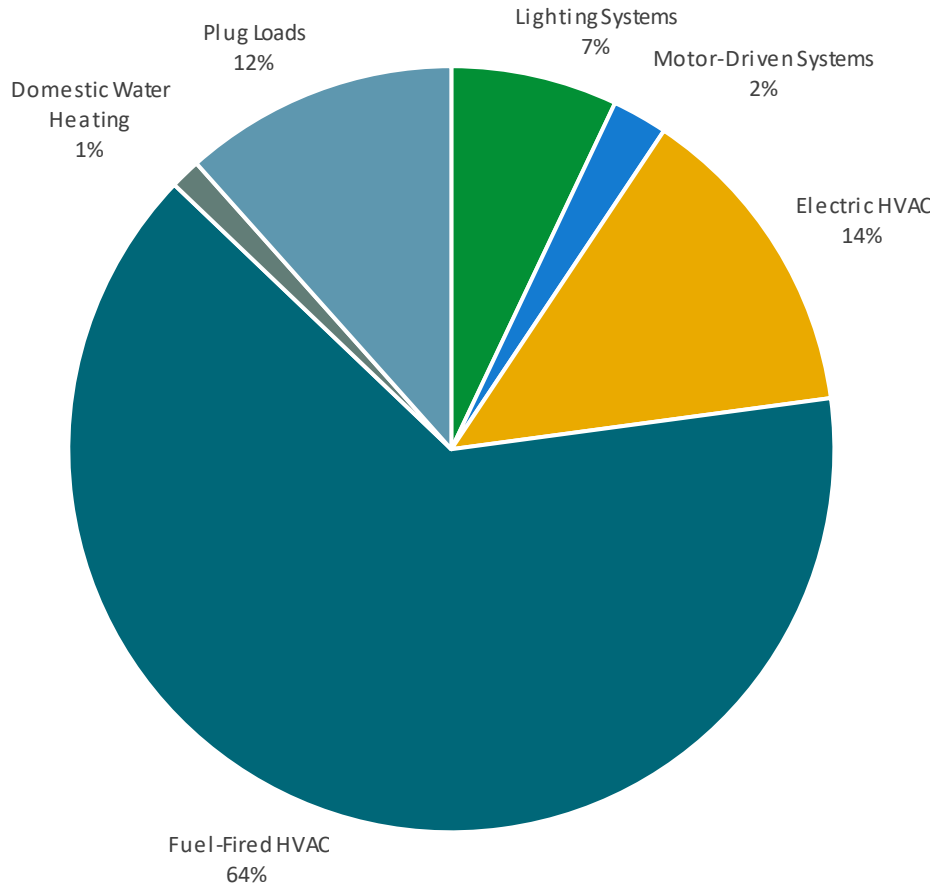
Figure 5 - Energy Balance
