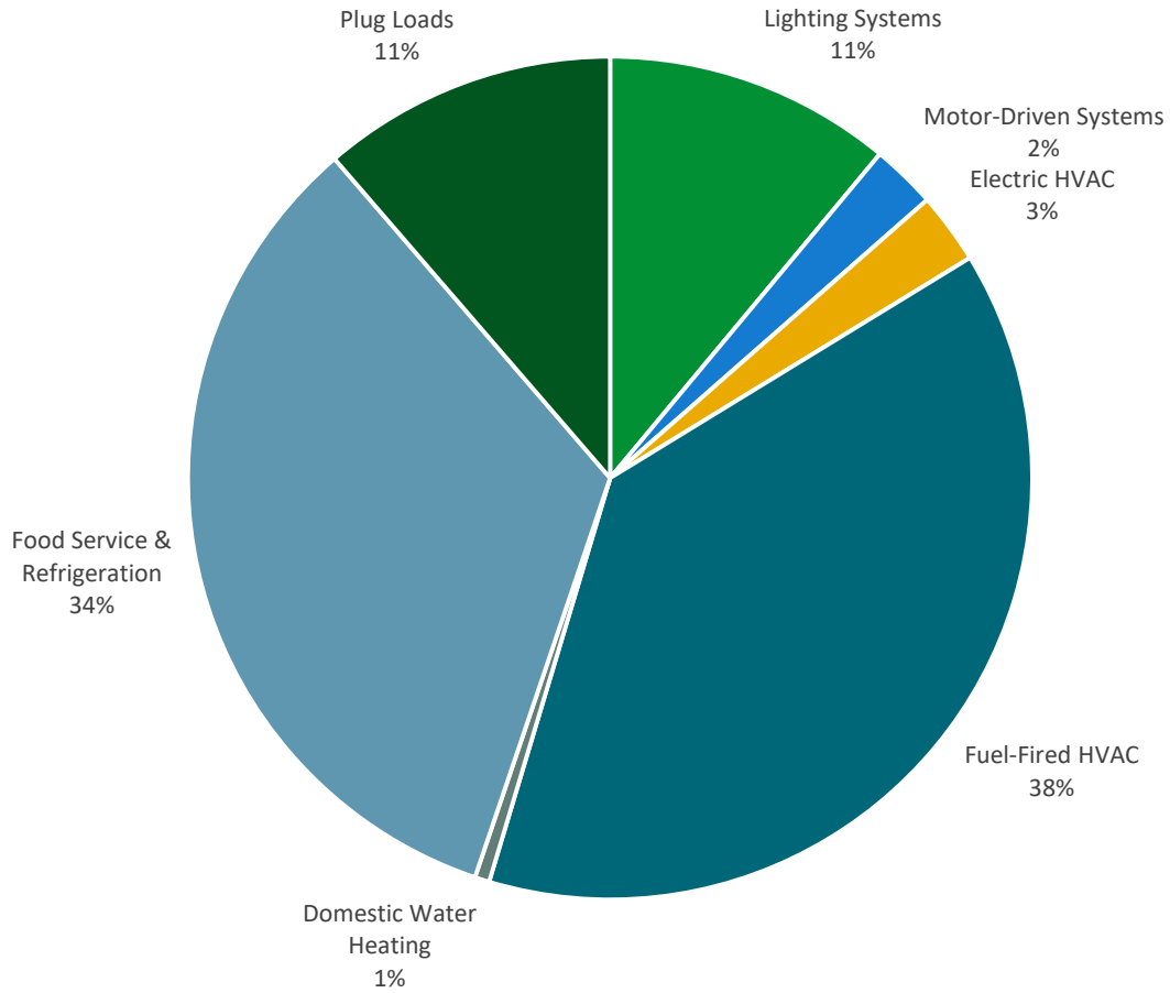
Figure 5 - Energy Balance
