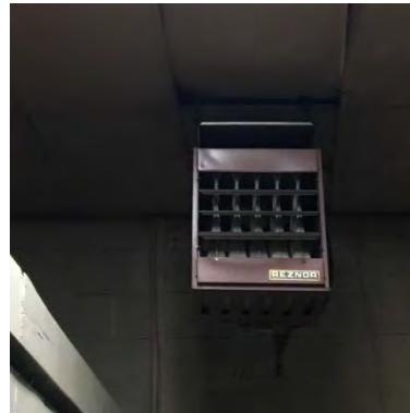
Image # - Unit heater
