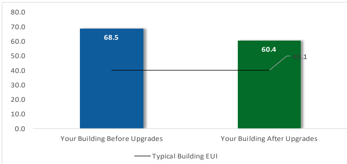
Figure 6 - Energy Use Intensity Comparison
