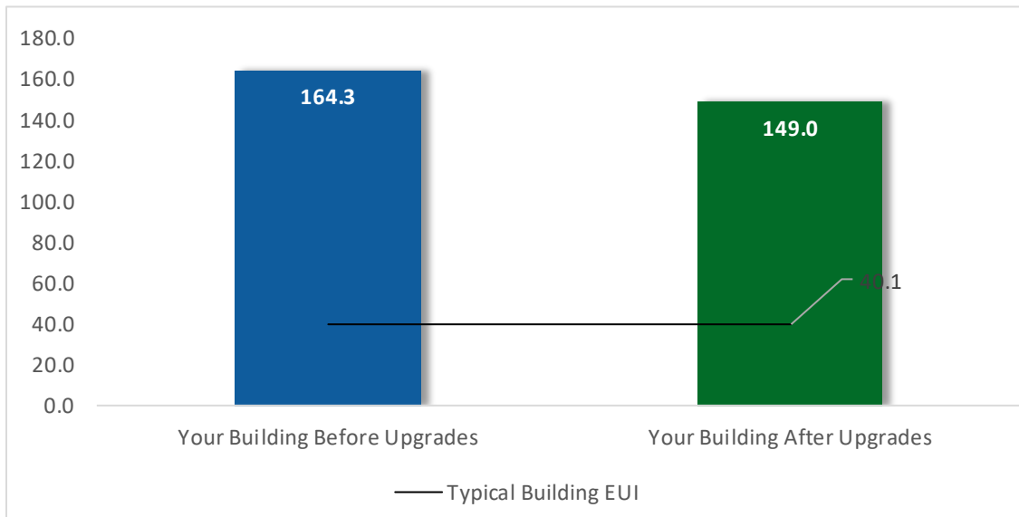
Figure 8 - Energy Use Intensity Comparison
