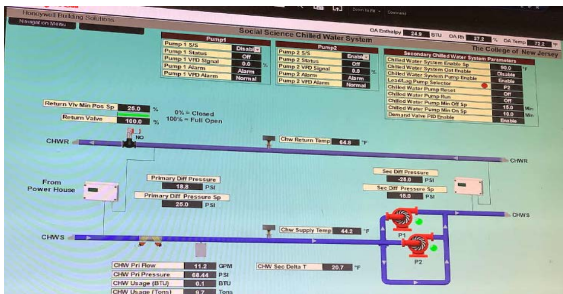
Chilled Water EMS Diagram View
