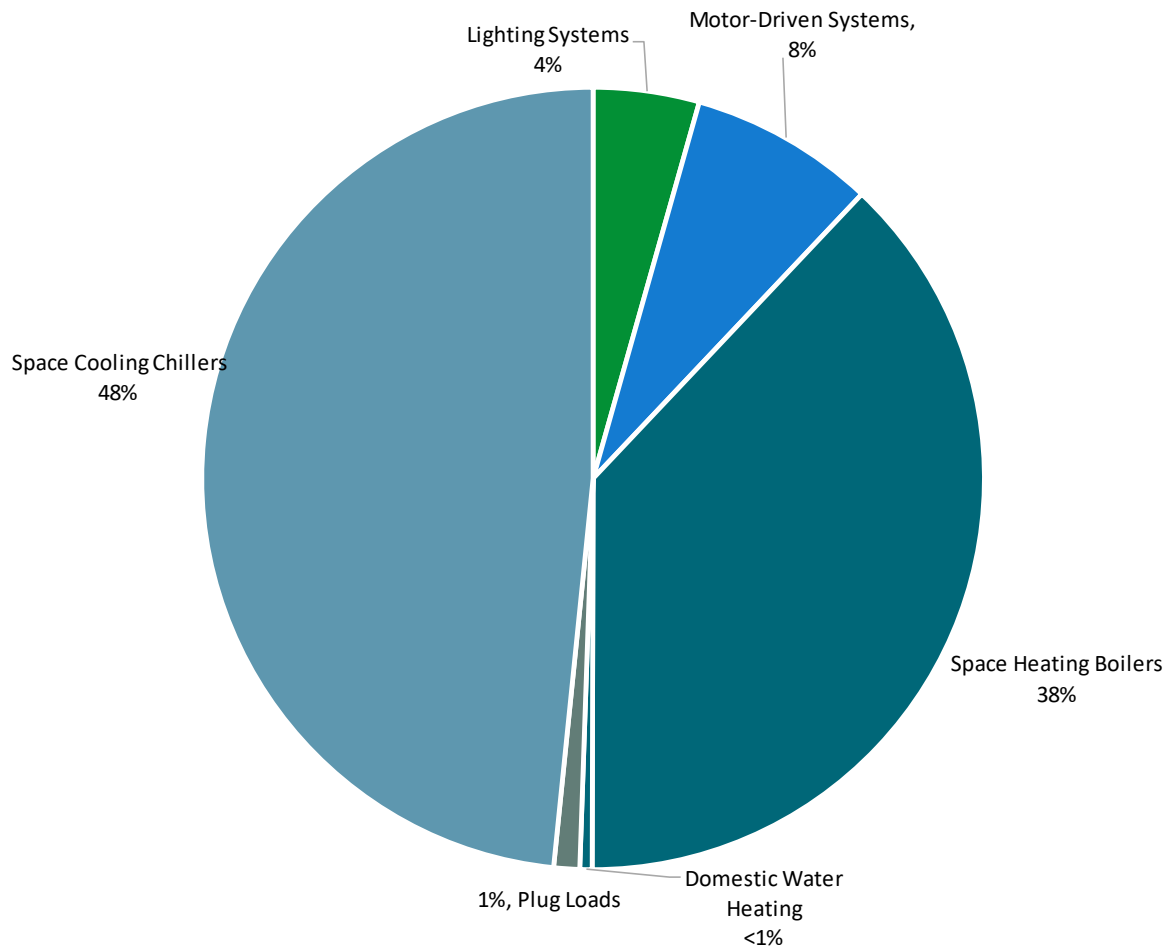
Figure 5 - Energy Balance
