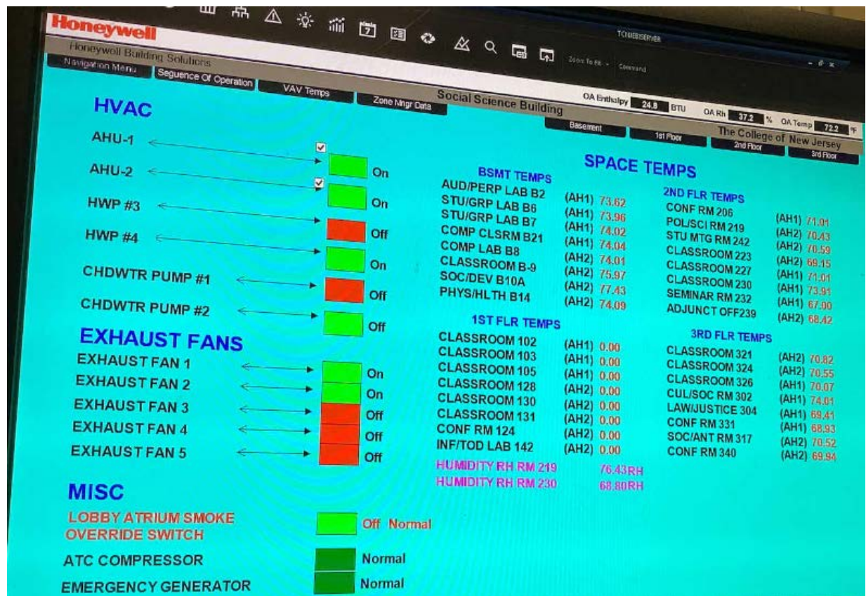
EMS Main Page
