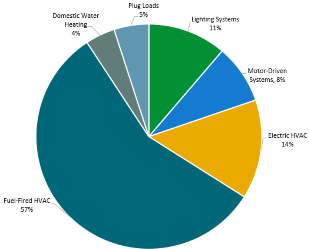
Figure 5 - Energy Balance
