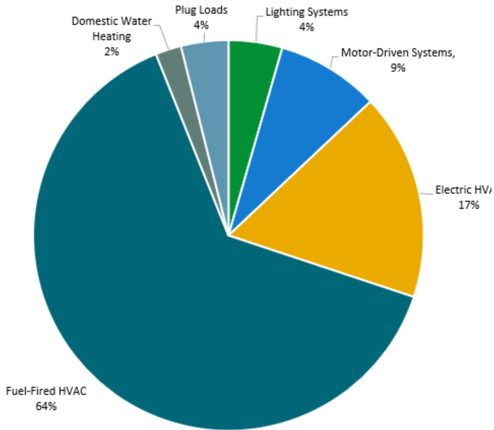
Figure 5 - Energy Balance
