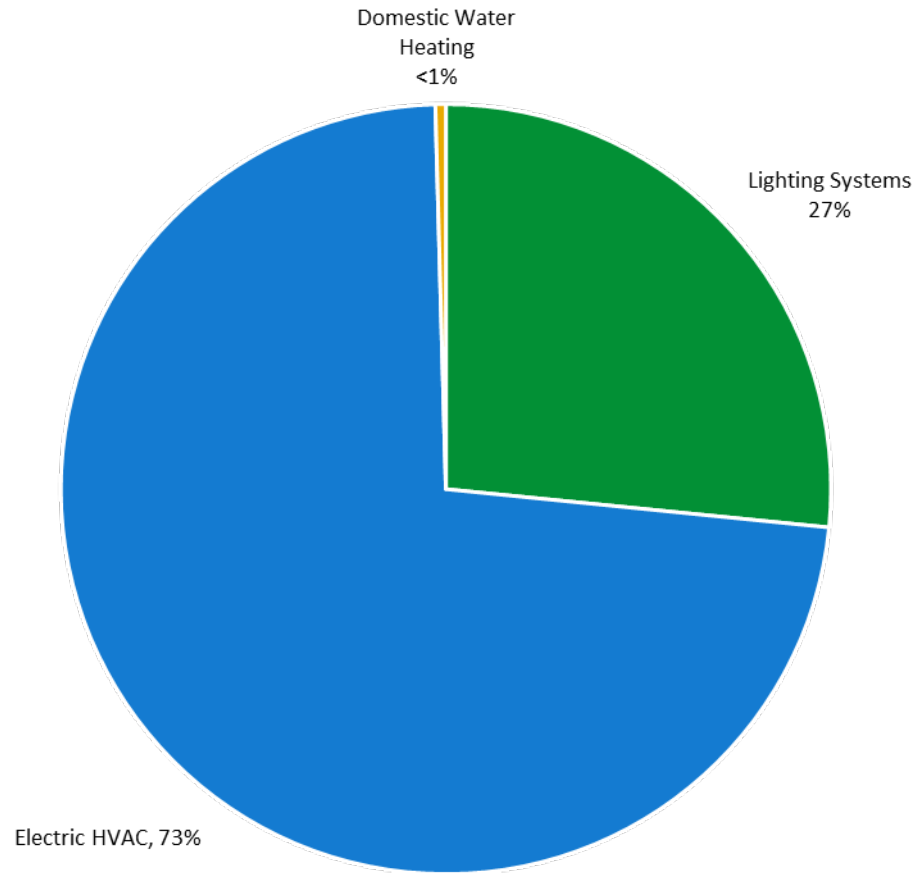
Figure 5 - Energy Balance
