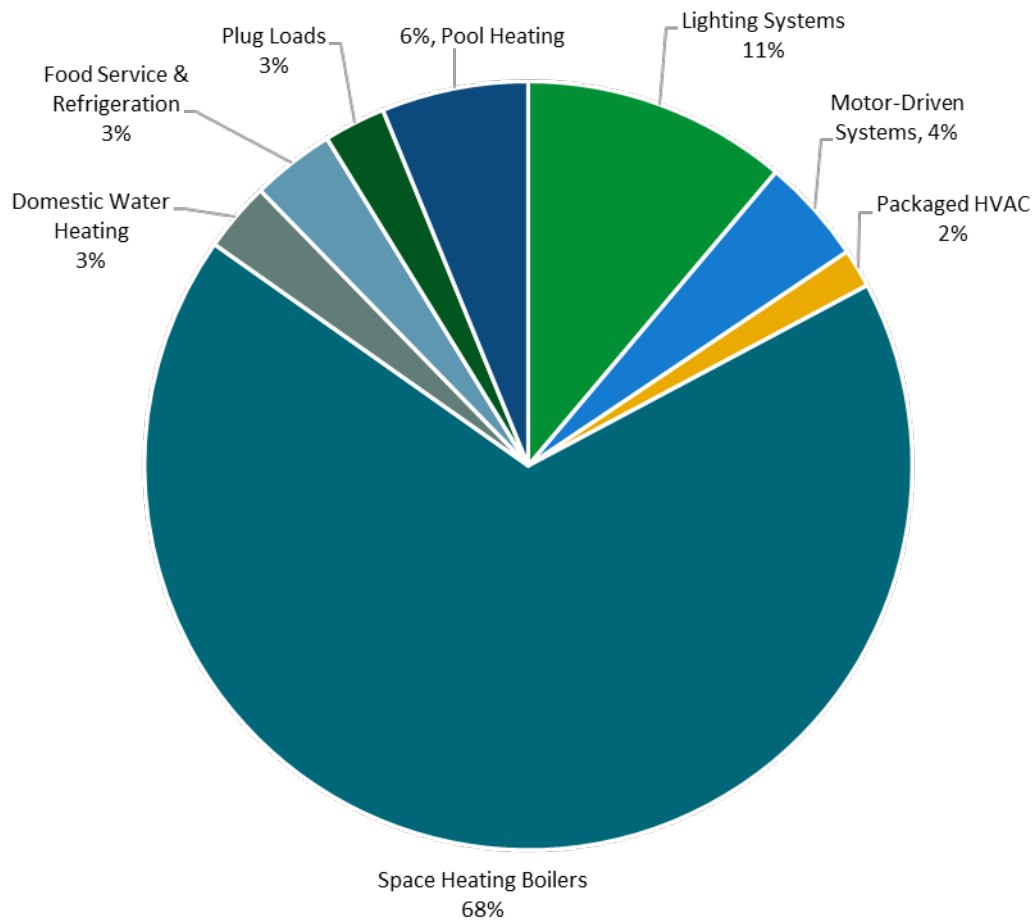
Figure 4 - Energy Balance
