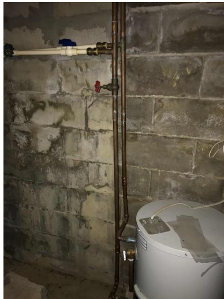
Storage Water Heater and Uninsulated DHW Pipes
