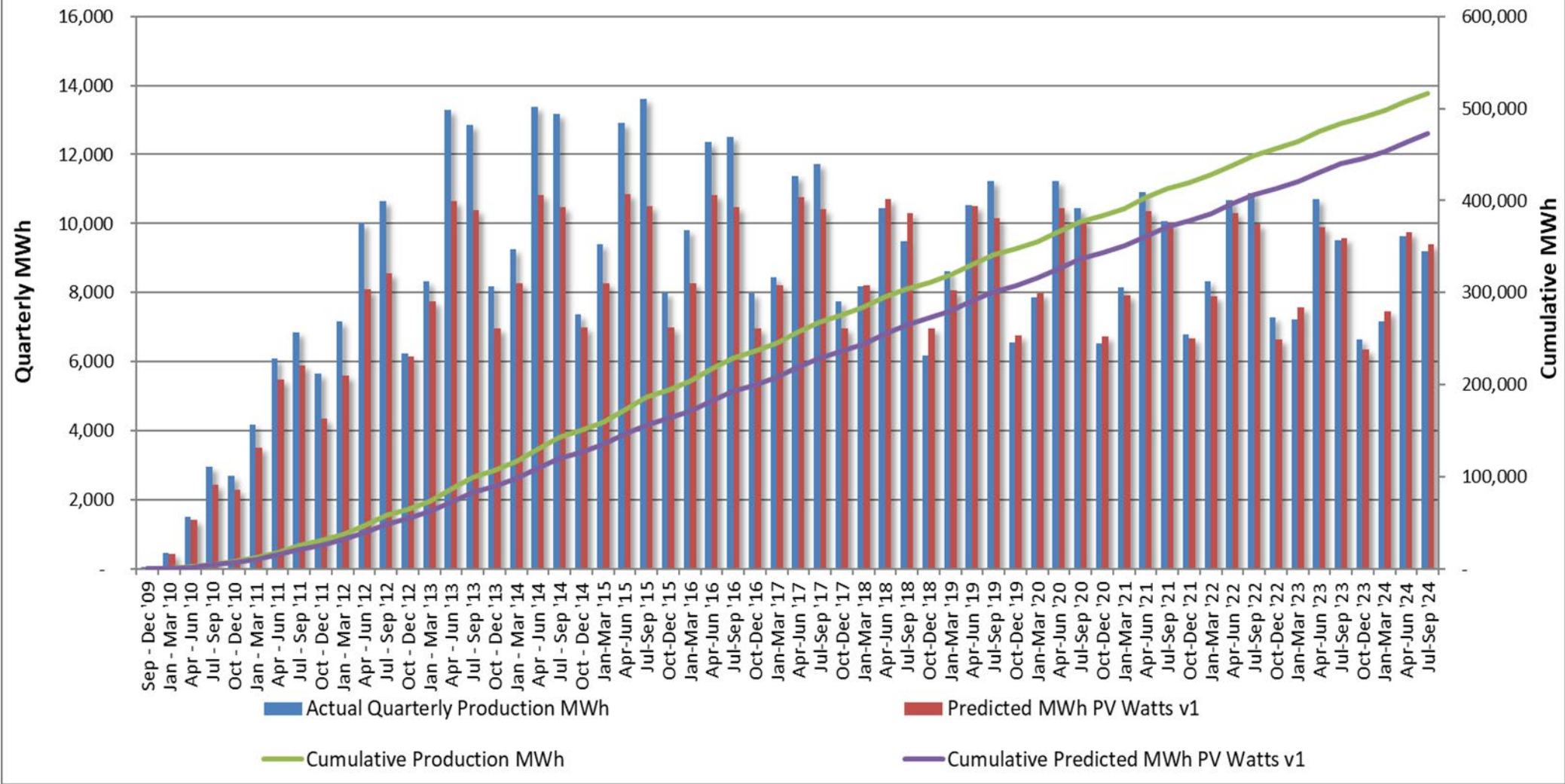
PSE&G Pole-Attached Solar: Quarterly Performance vs. PV Watts
